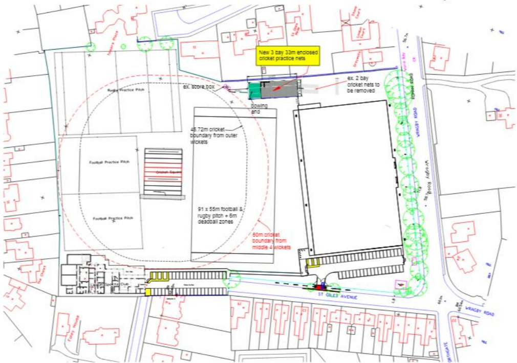
PROPOSED SITE PLAN 1:500
